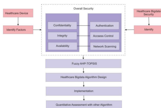
Fig. 1. Fuzzy AHP-TOPSIS approach for healthcare big data security.
