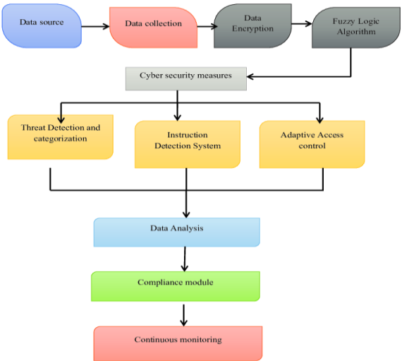
Fig. 3. Fuzzy logic-based cybersecurity framework.
